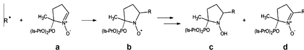
Figure 1. The general trapping chemistry of the DIPPMPO spin trap system.
