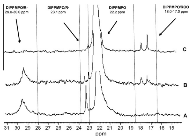
Figure 2. ^{31}\text{P} NMR spectra of DIPPMPO after reaction with linoleic acid in the presence of lipoxygenase. (A) In a glass vial with air saturated buffer and head space filled with argon; (B) in air without stirring; and (C) with a continuous air stream and stirring.
